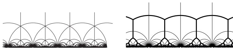
FIGURE 1. The figure on the left shows the usual fundamental domain in \mathbb{H} for the action of \mathrm{SL}_2(\mathbb{Z}) . On the right is the trivalent tree of well-rounded binary quadratic forms (shown in bold ) with dual tessellation by ideal hyperbolic triangles.
