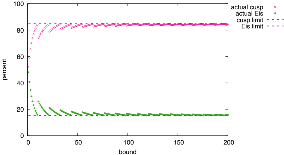
Cuspidal and Eisenstein Percentages for N = 11
