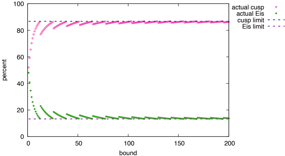
Cuspidal and Eisenstein Percentages for N = 13
