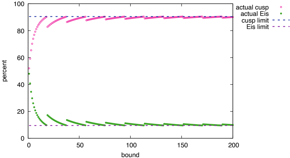
Cuspidal and Eisenstein Percentages for N = 19
