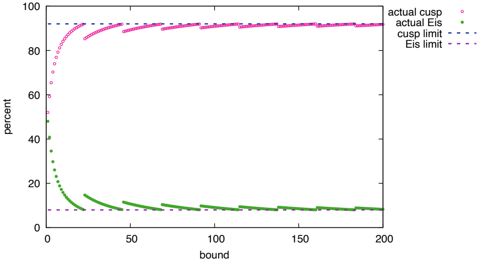
Cuspidal and Eisenstein Percentages for N = 23
