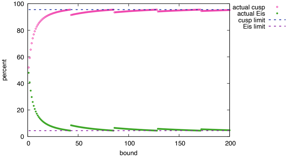
Cuspidal and Eisenstein Percentages for N = 43
