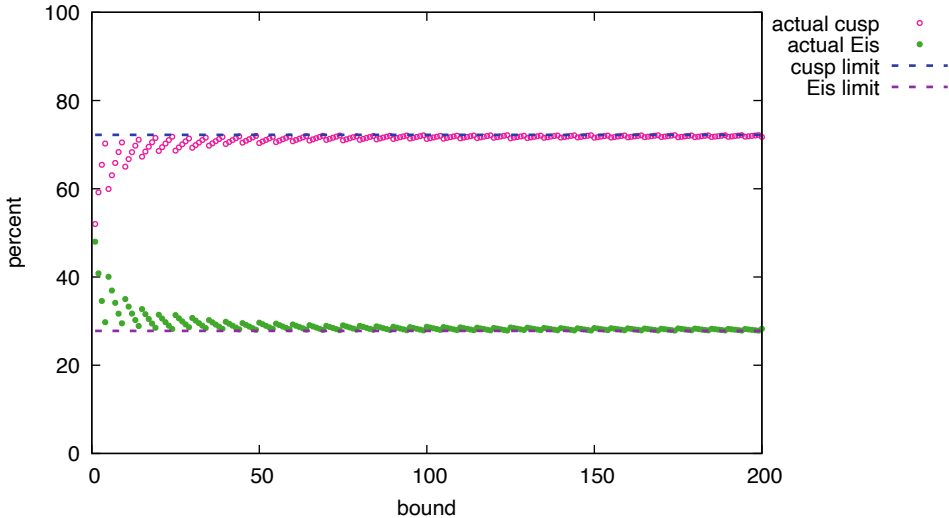
Cuspidal and Eisenstein Percentages for N = 5
