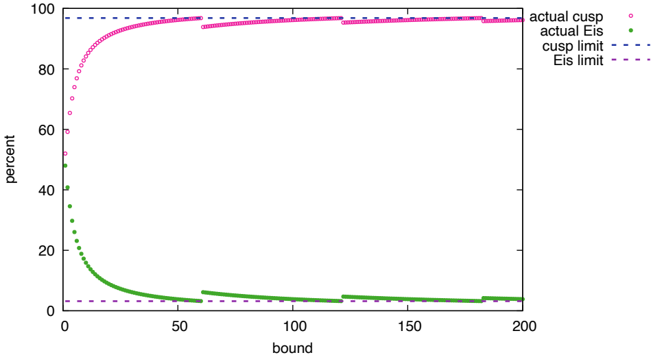
Cuspidal and Eisenstein Percentages for N = 61
