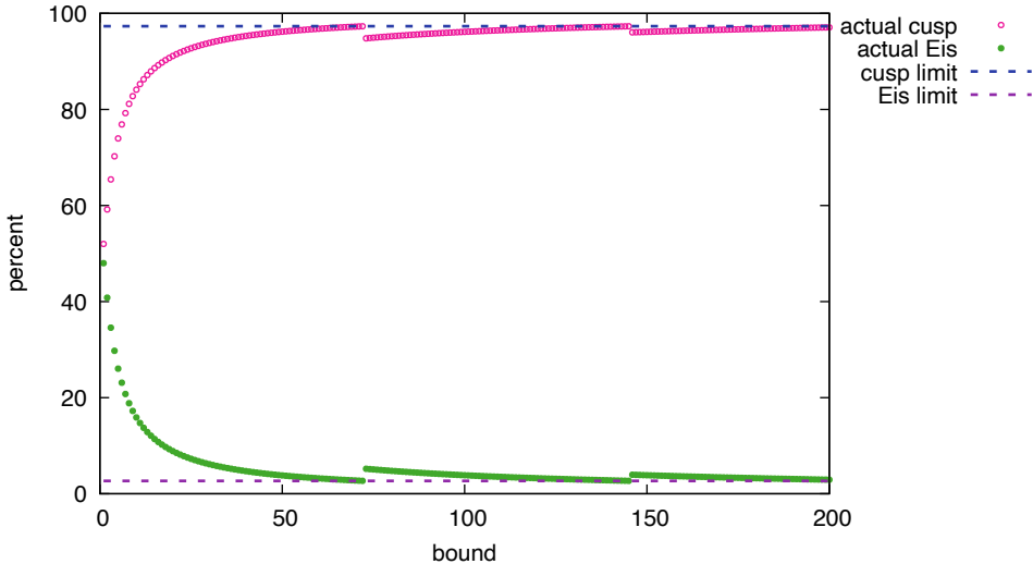
Cuspidal and Eisenstein Percentages for N = 73
