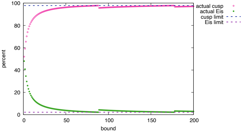
Cuspidal and Eisenstein Percentages for N = 89
